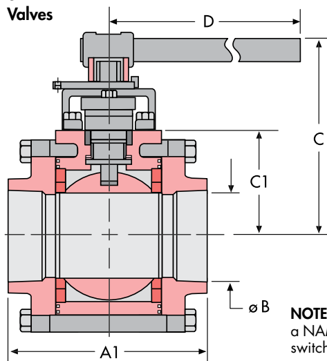
3" – 4" Valves
