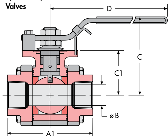
1/4" – 2 1/2" Valves
